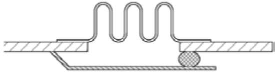
Packed Bellows
